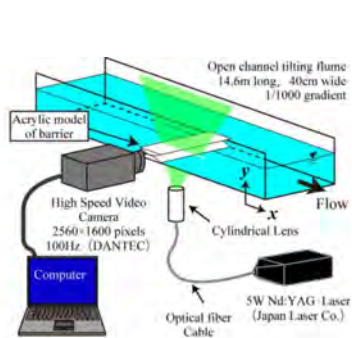
(a) Experimental apparatus
